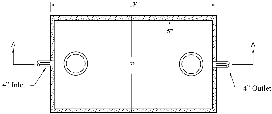
PLAN VIEW
